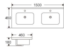
Cabinet basin Above cabinet mounting BH4615D 1500x460x180 mm
