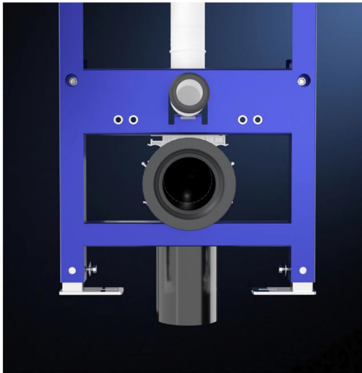
FIXATION FEET
