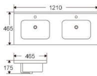
Cabinet basin Above cabinet mounting BG4612D 1210x465x175mm
