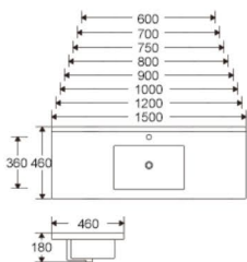
BH3660 Size: 600x360x180mm BH4660 Size: 600x460x180mm BH4670 Size: 700x460x180mm BH4675 Size: 750x460x180mm BH4680 Size: 800x460x180mm BH4690 Size: 900x460x180mm BH4610 Size: 1000x460x180mm BH4612 Size: 1200x460x180mm BH4615 Size: 1500x460x180mm
